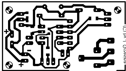
thermostat_mit_tiny13_und_relais.cdr
